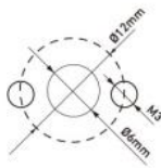
Propeller Mounting Hole
