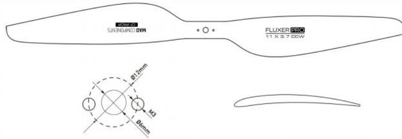
Propeller Mounting Hole
