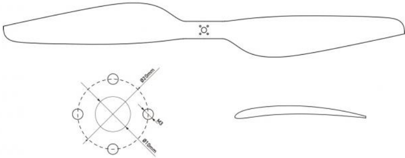
Propeller Mounting Hole
