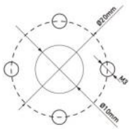
Propeller Mounting Hole
