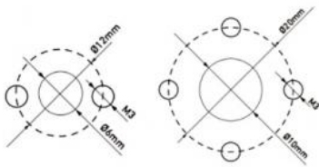
Propeller Mounting Hole
